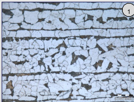
uninfluenced base metal
