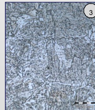
coarse grainulation
