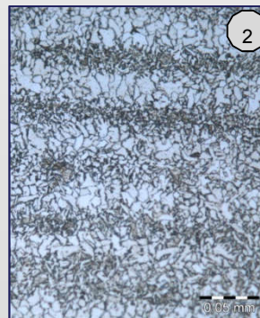
perlite dissolution
